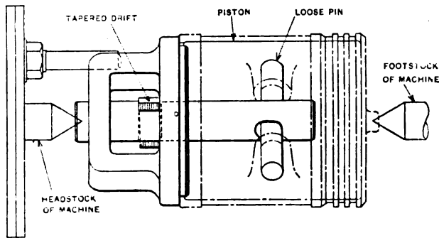
Grinding fixture with mounted piston
